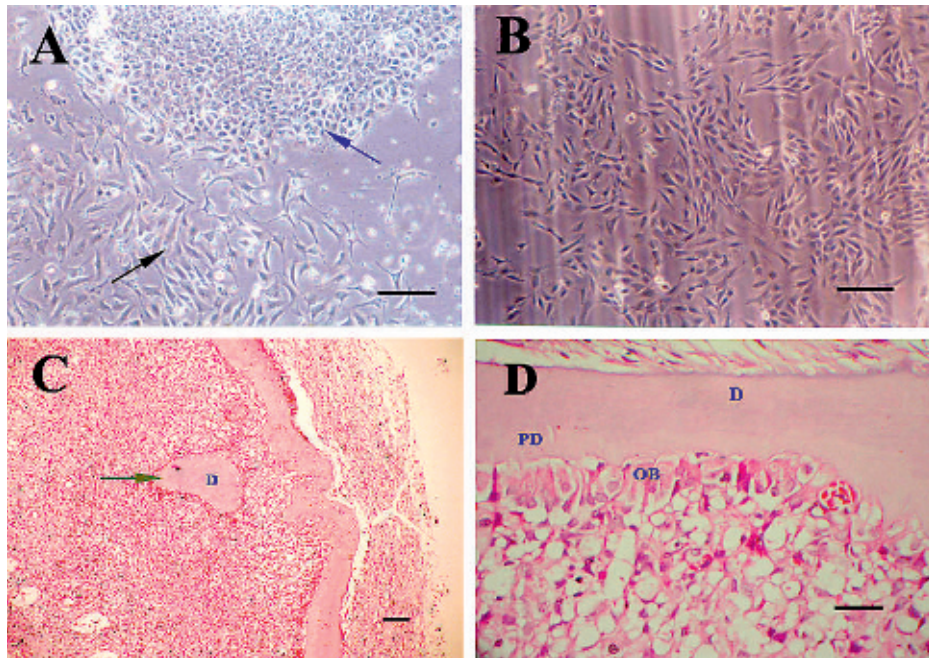
Fig 2A to D Tooth-forming potentiality of tooth germ cells (TGCs).
