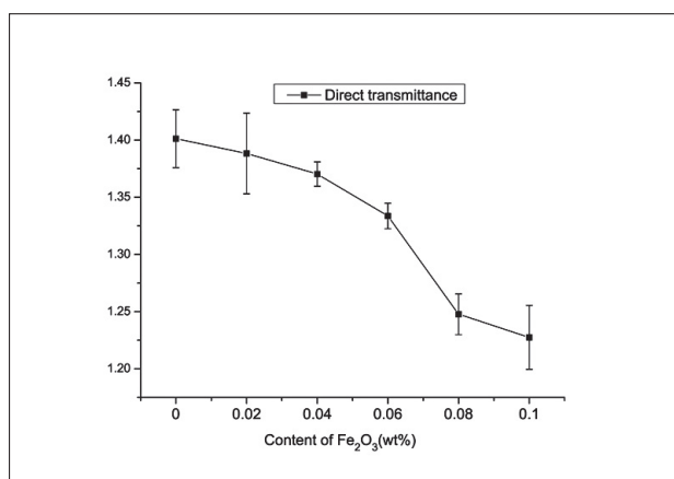
Fig 3 The direct transmittance of specimens with different amounts of \text{Fe}_2\text{O}_3 .
