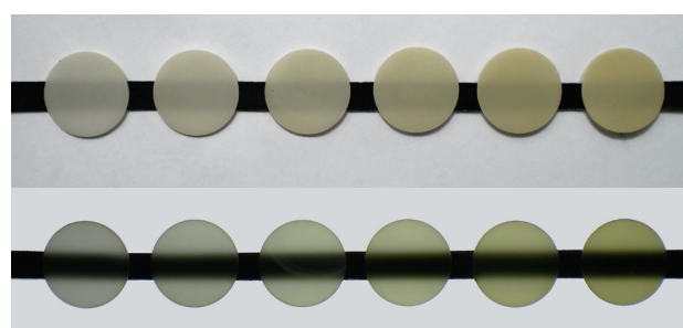
Fig 1 Glazed specimens with different amounts of Fe 2 O 3 on a black and white background with reflected and transmitted light. From left to right: 0 wt%, 0.02 wt%, 0.04 wt%, 0.06 wt%, 0.08 wt% and 0.10 wt%.
