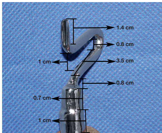
Fig 2 U shank with dimensions and a tip, with a concave surface.
